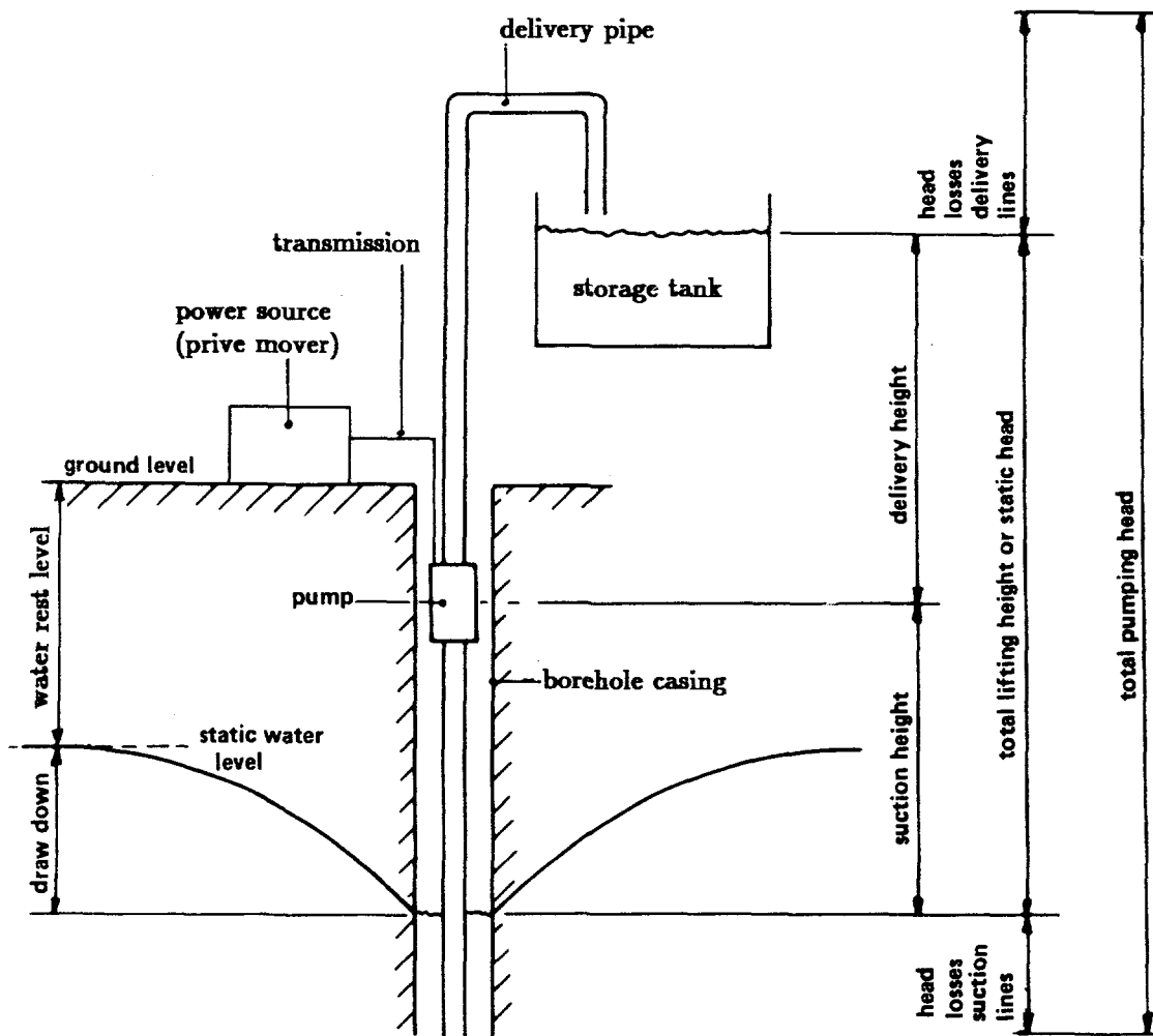
Figure 1.3.b. Composition of total pumping head.
