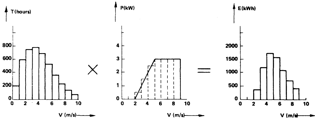
Figure B.3. Calculation of total output of a wind machine from the wind speed frequency distribution and the output curve (reference 3).
