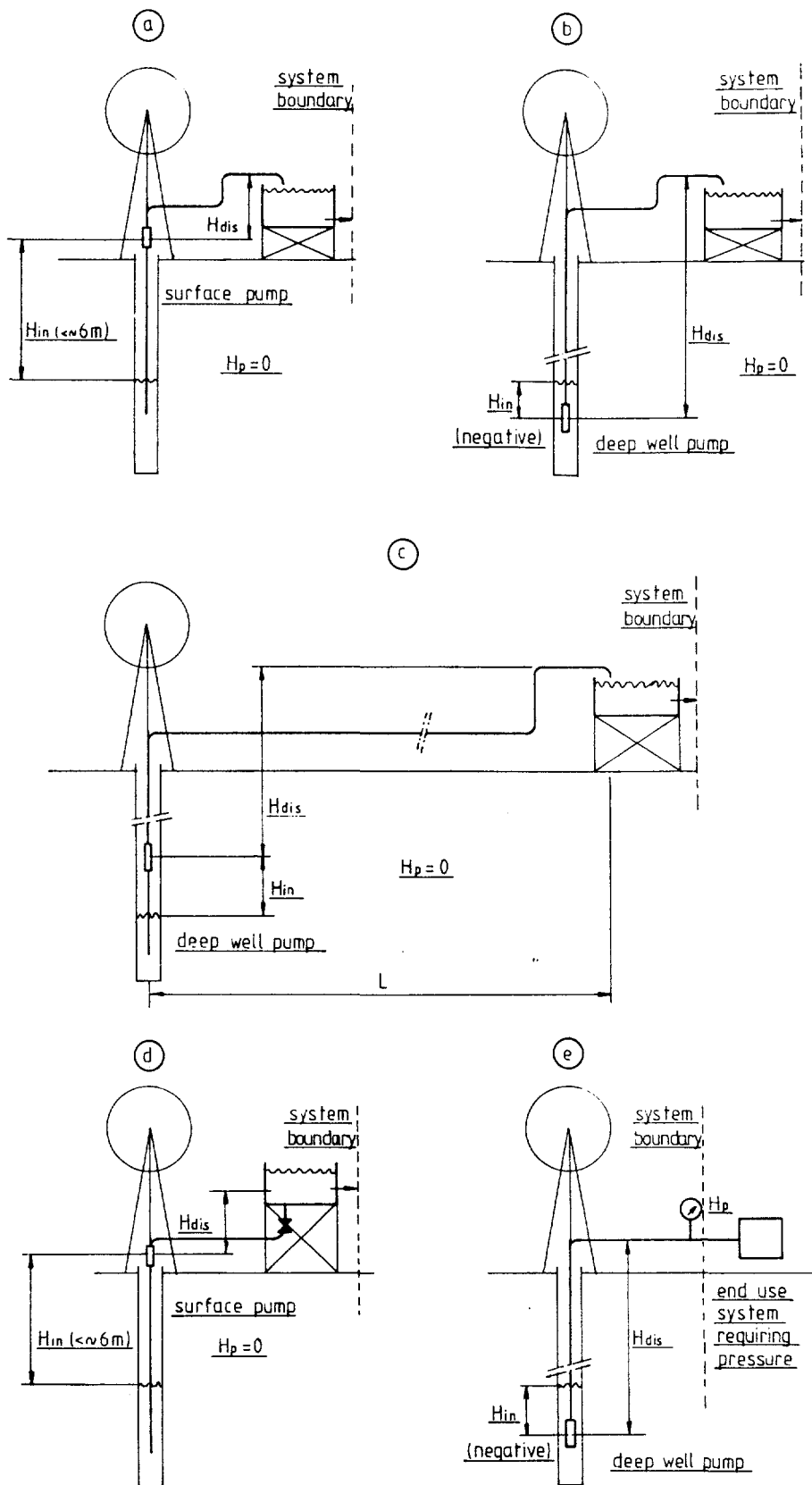
Figure 5.1. Examples of head measurements.
