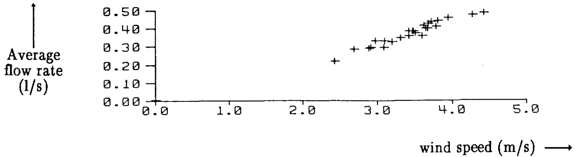
Figure 4.1. Example of water output curve
