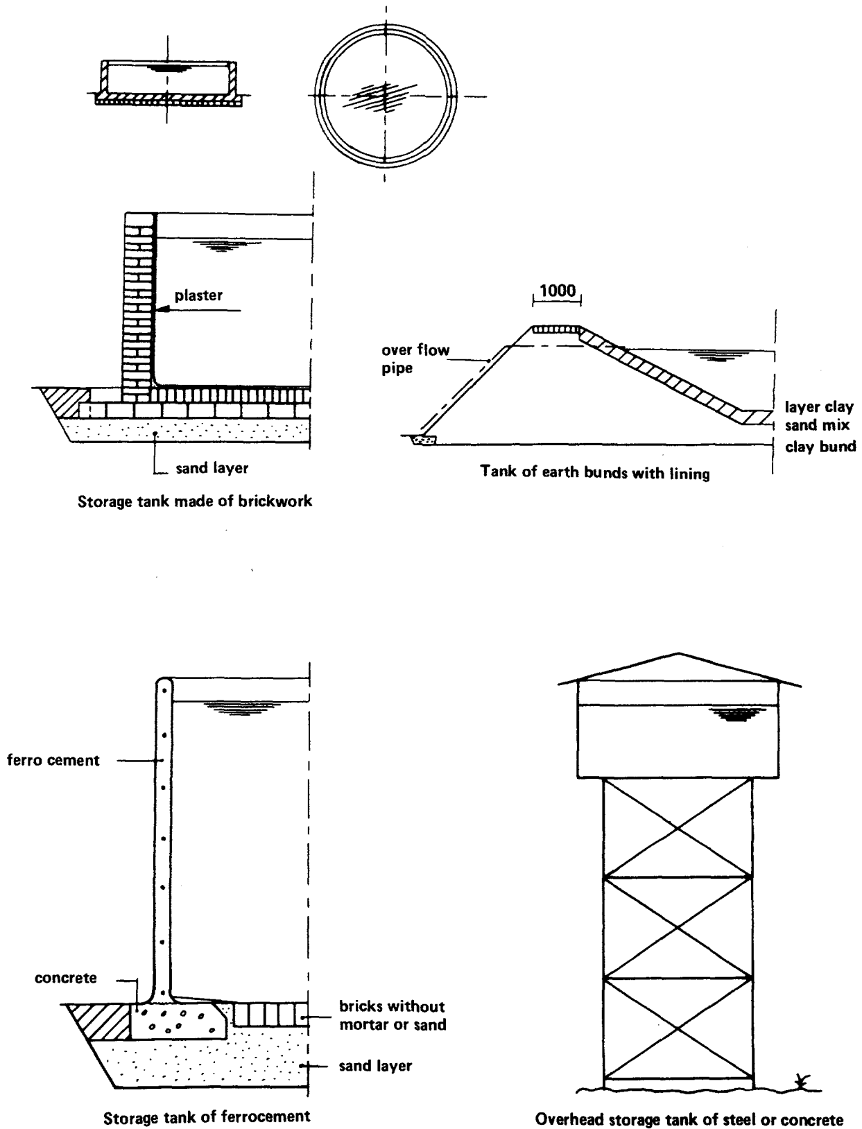
Figure 2.10. Storage tanks: principles of construction.
