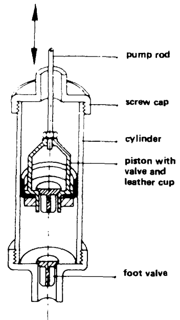
Components of a screw cap pump
