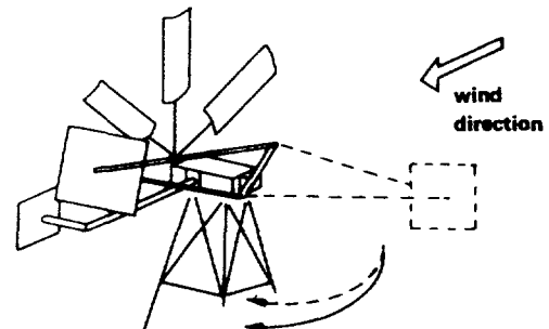
Hinged vane safety system
