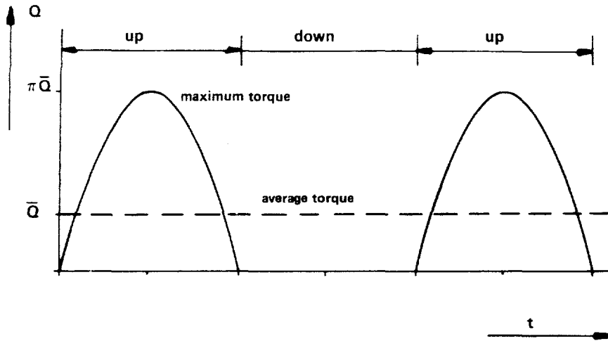
Figure 2.7. Torque of a piston pump versus time.
