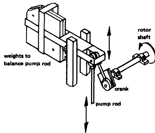
Direct drive transmission
