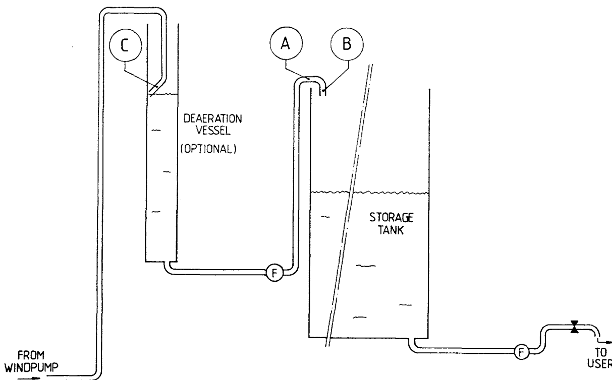
Figure 2.1. Installation of flow meters
