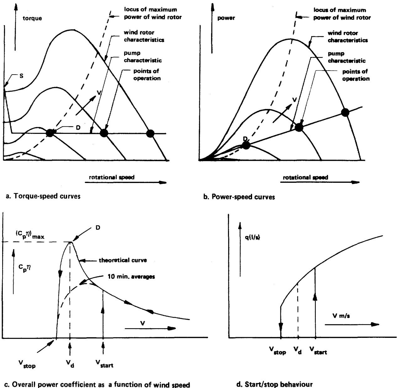
Figure 2.9. Matching of windmill and piston pumps.
