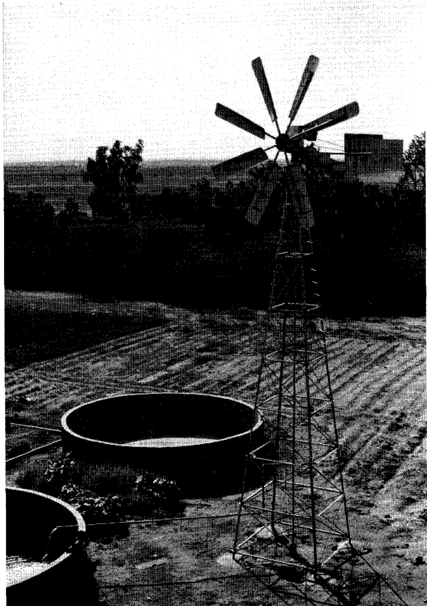
In specifying the wind pump all items should be included: water source, wind pump, delivery system, storage system and distribution or field application system. Soba experimental farm, Sudan 1987.
