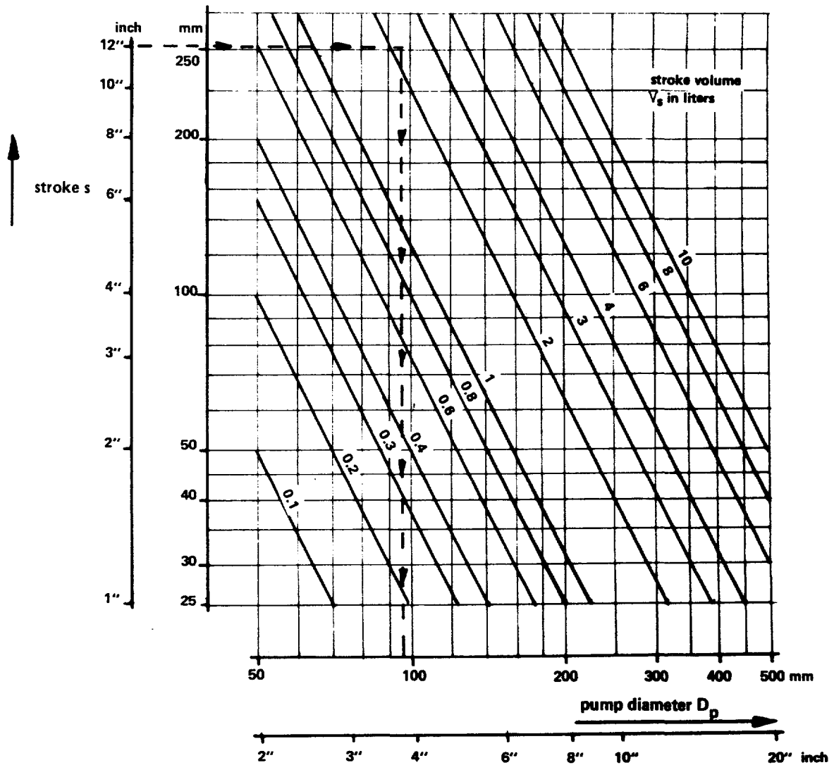
Figure 3.5. Nomogram to choose stroke and diameter of piston pump.
