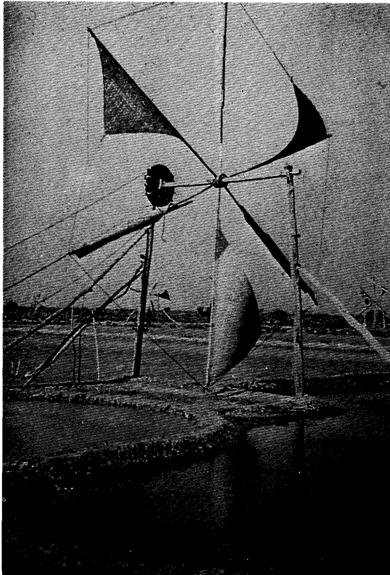
Local design of low head wind pump in Thailand, used for pumping water into salt ponds.
