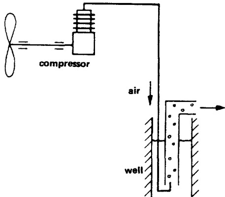
Windmill with a pneumatic transmission, driving an air lift pump: no moving parts in the well
