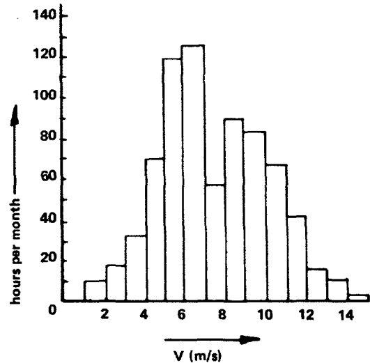
d. The velocity frequency data for Praia airport, Cape Verde (June 1975), in a histogram
