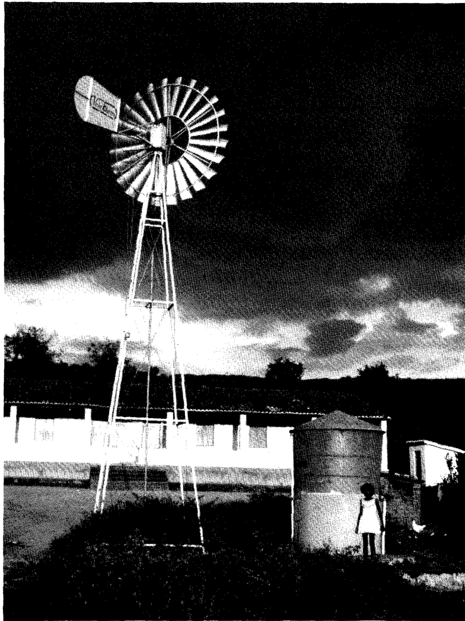
Water supply of a small community in the dry interior of Paraíba state, Brazil, by means of a Vida Eterna wind pump of conventional design.
