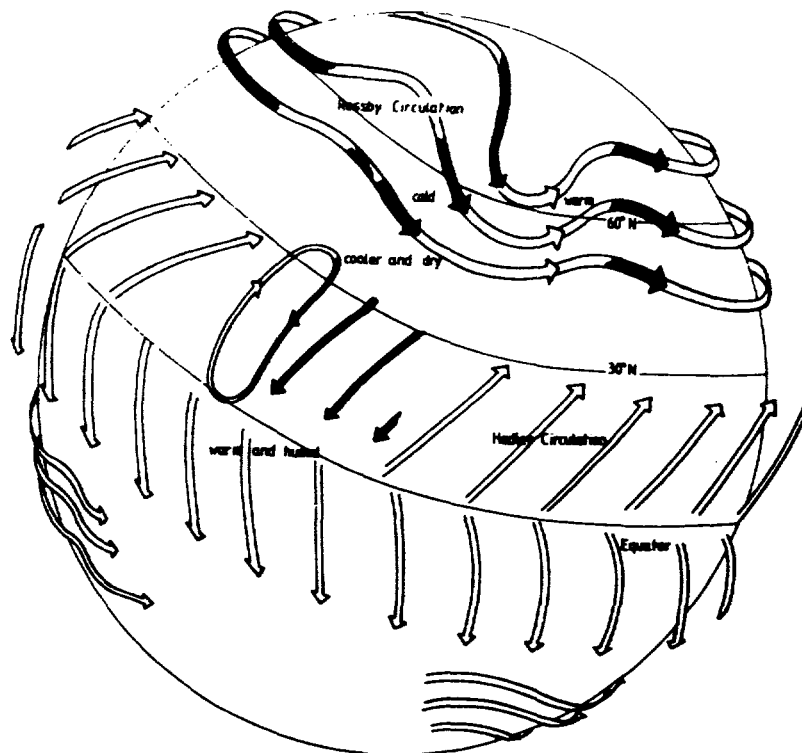
Figure A.1. Schematic picture of the general circulation of air around the globe. North and South of 30° N and 30° S, respectively, a westerly circulation persists, while in the tropics one finds NE and SE trade winds (reference 7).
