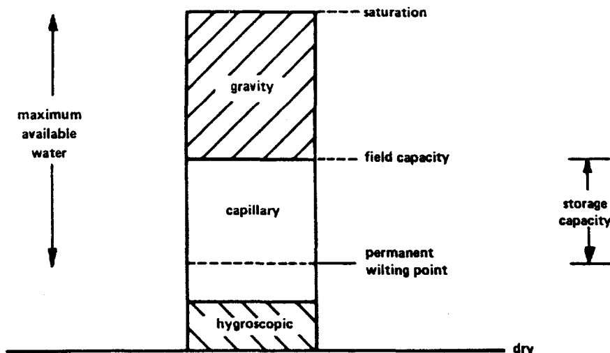
Figure 3.2.a. Soil moisture quantities (reference 1).
