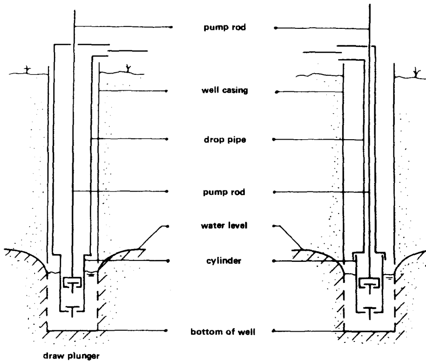
Deep well pump arrangement
