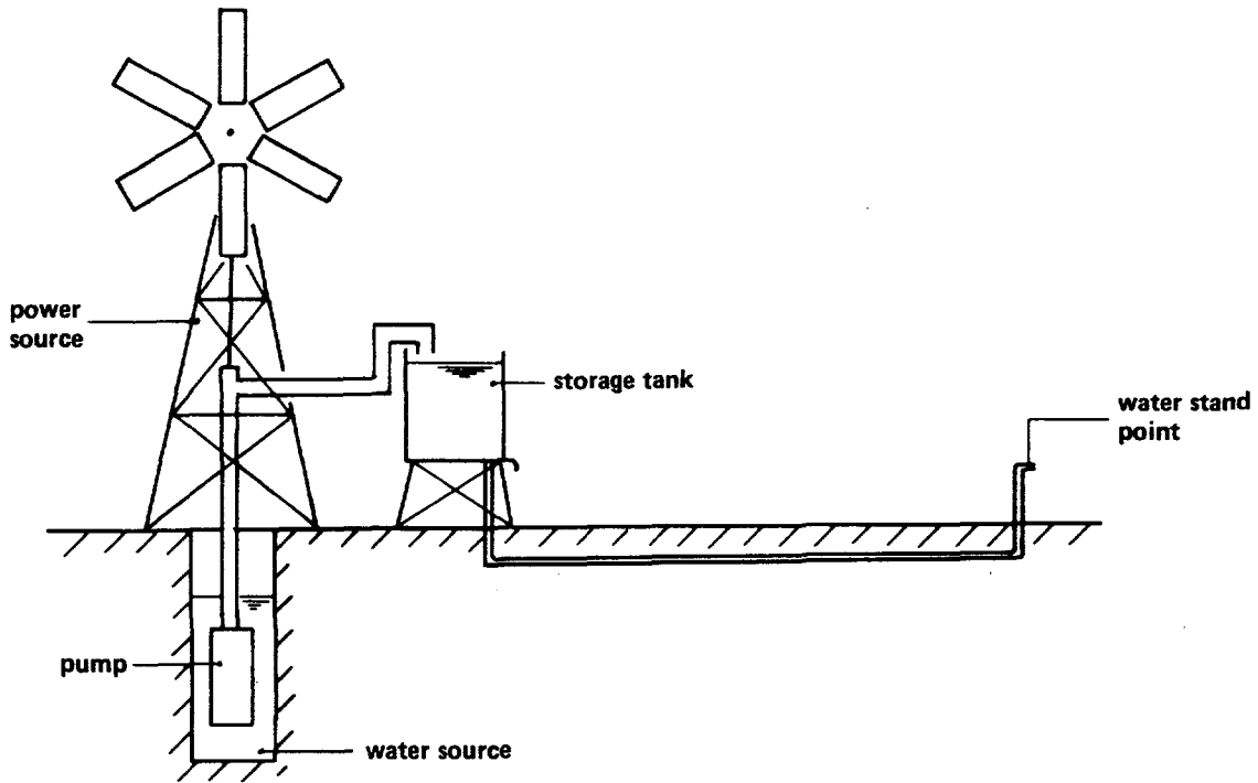
Figure 1.2.a. Schematic layout of a village water supply system showing the five major components.
