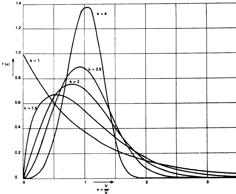
Figure A.8. The Weibull distribution.
