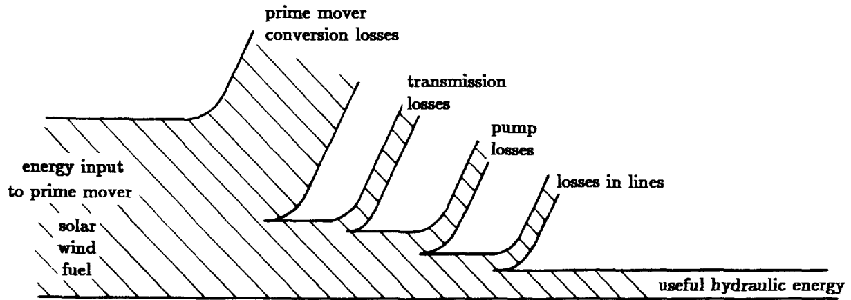
Figure 1.3.a. Energy losses in a water pumping system.
