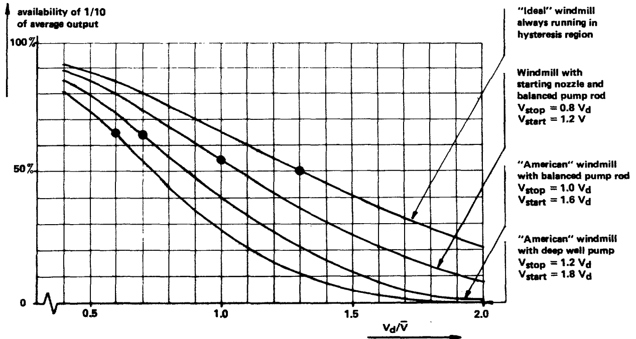
Figure B.2. Output availability of 10% of average output as a function of design wind speed over average wind speed. Dots: reasonable design according to Table 2.2, Chapter 2.
