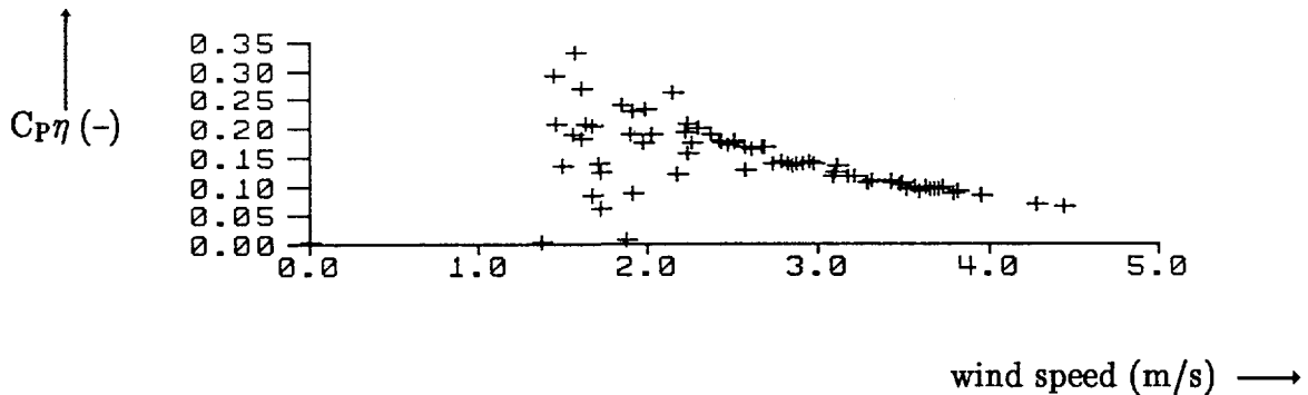
Figure 4.3. Example of overall windpump performance factor curve.
