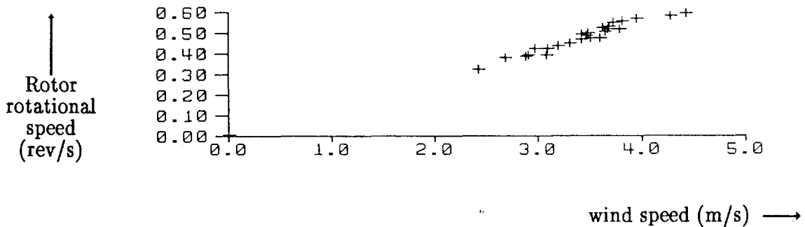
Figure 4.2. Example of rotor rotational speed curve.
