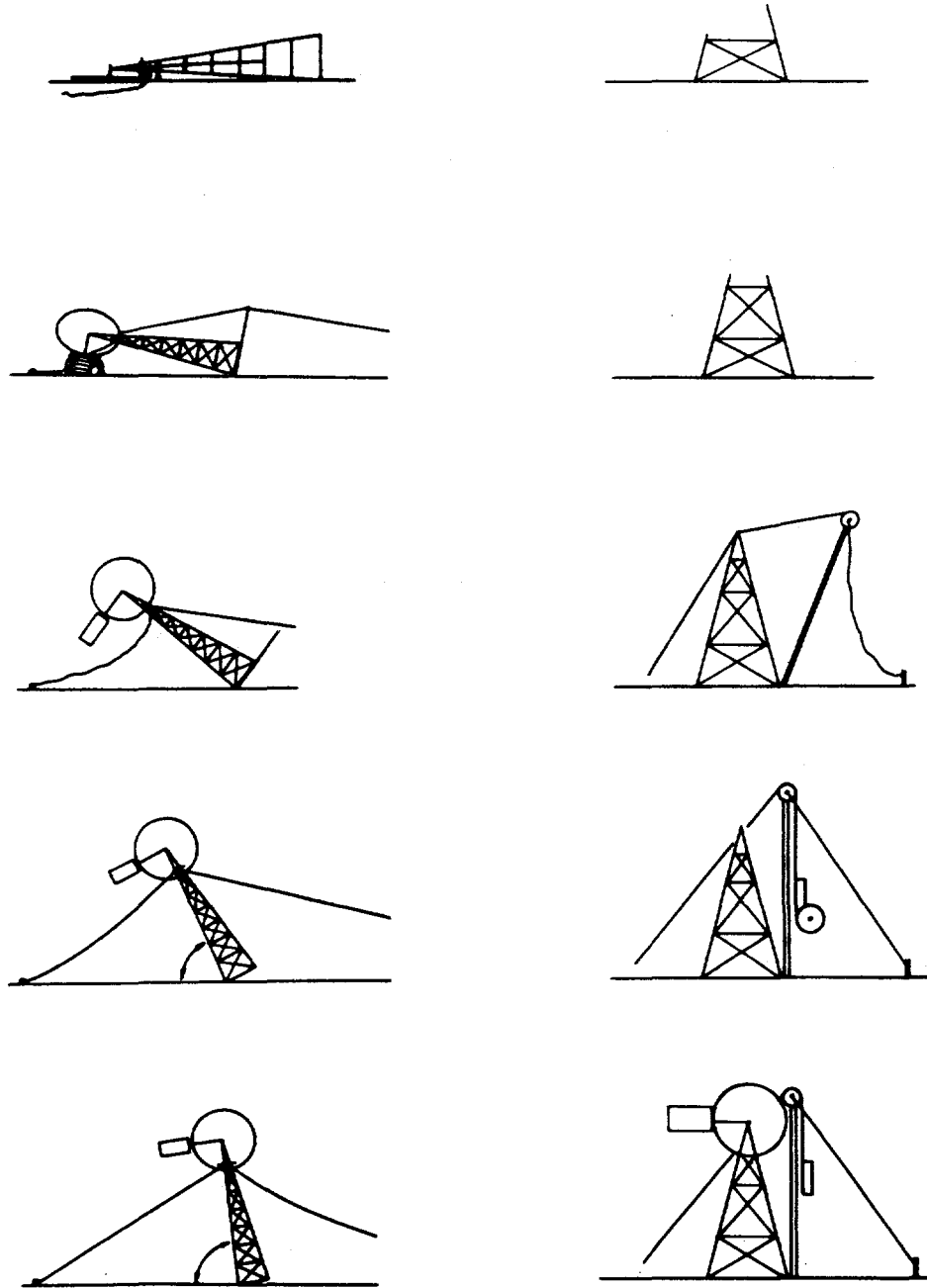
6.2.b Assembly from ground level upwards
