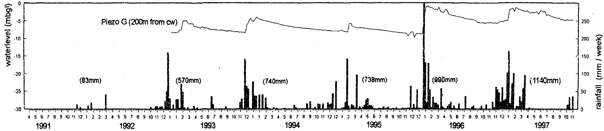
Figure 7.1 Romwe collector well performance, 1991-97
