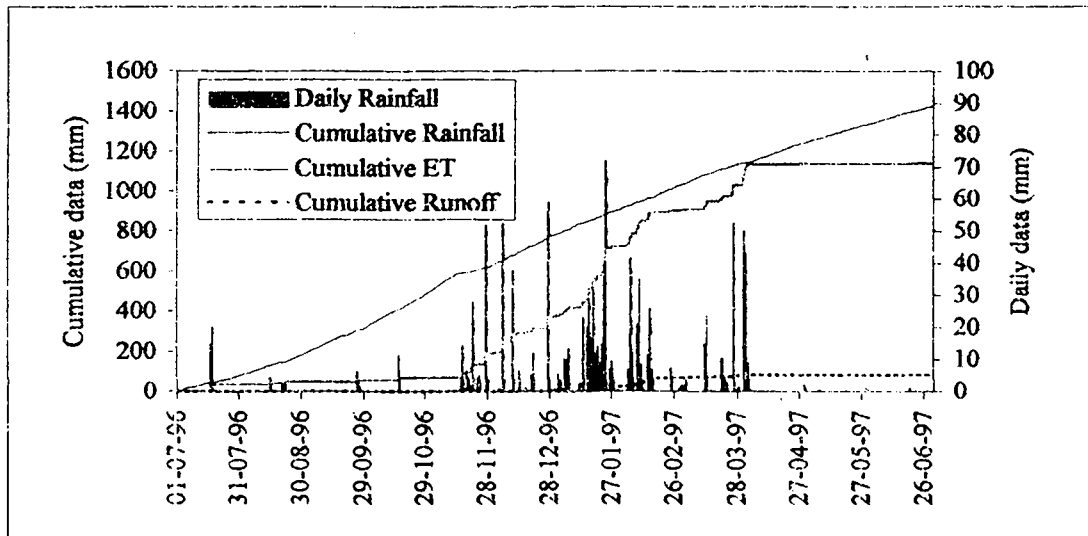
Figure 6.1 Total and daily rainfall, potential evaporation (Penman, 1948) and catchment runoff a) 1994/95, b) 1995/96, c) 1996/97
