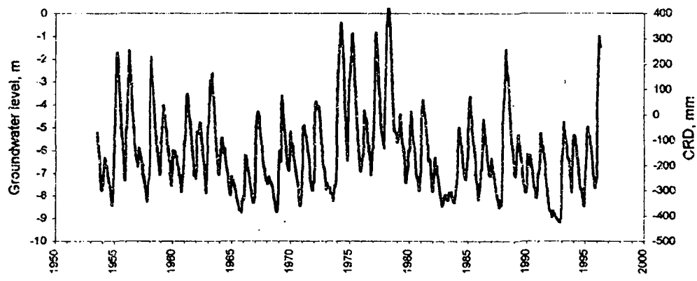
Figure 5.2 Simulated groundwater levels, 1952-96, a) ACRU, b) ACRU including surface redistribution of rainfall, c)CRD 1:12
