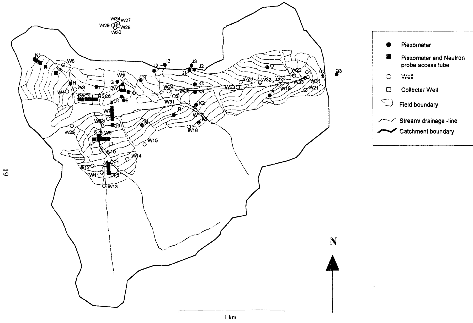
Figure 2.4b Groundwater and soil moisture monitoring sites
