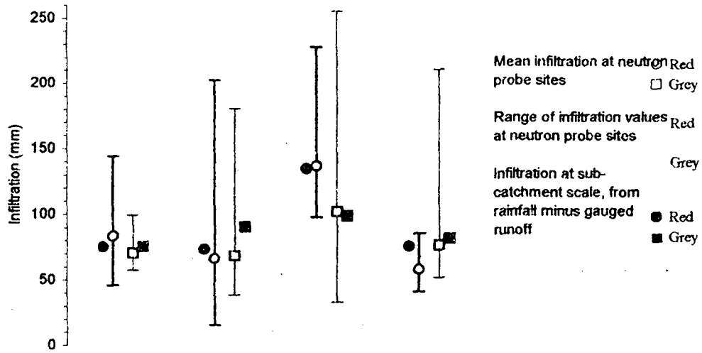
a) Infiltration at point and sub-catchment scales
