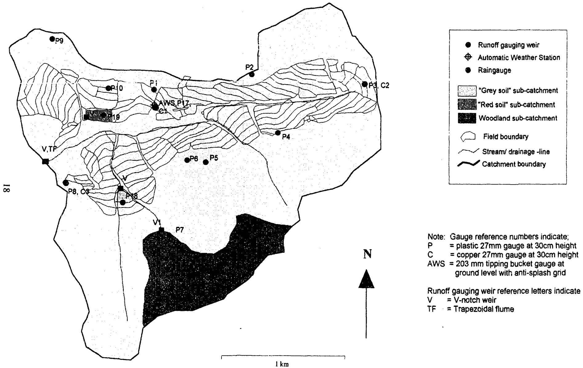
Figure 2.4a Gauging stations, sub-catchments and meteorological instrumentation
