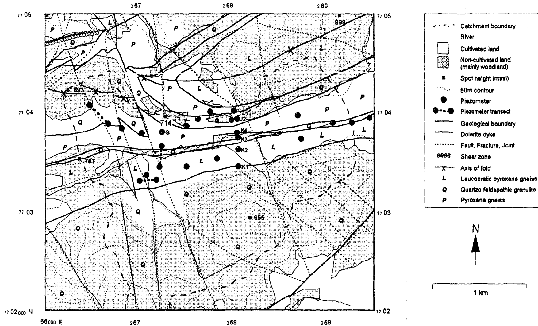
Figure 4.1 Catchment geology and monitoring sites
