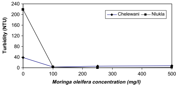
Fig. 3. Turbidity reduction of high turbid well water with M. oleifera .
