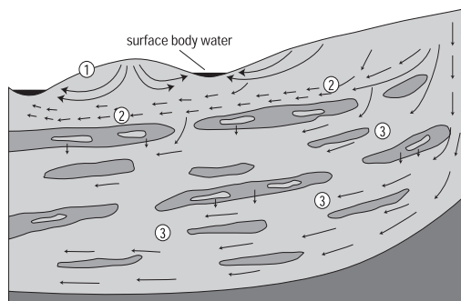
Figure 3.3. Thick sediments associated with rivers and coastal regions ■ High hydraulic conductivity aquifer ■ Low hydraulic-conductivity aquifer ← Direction of groundwater flow ① Local groundwater subsystem (months–decades) ② Subregional groundwater subsystem (10s–100s years) ③ Regional groundwater subsystem (100s–1000s years)
