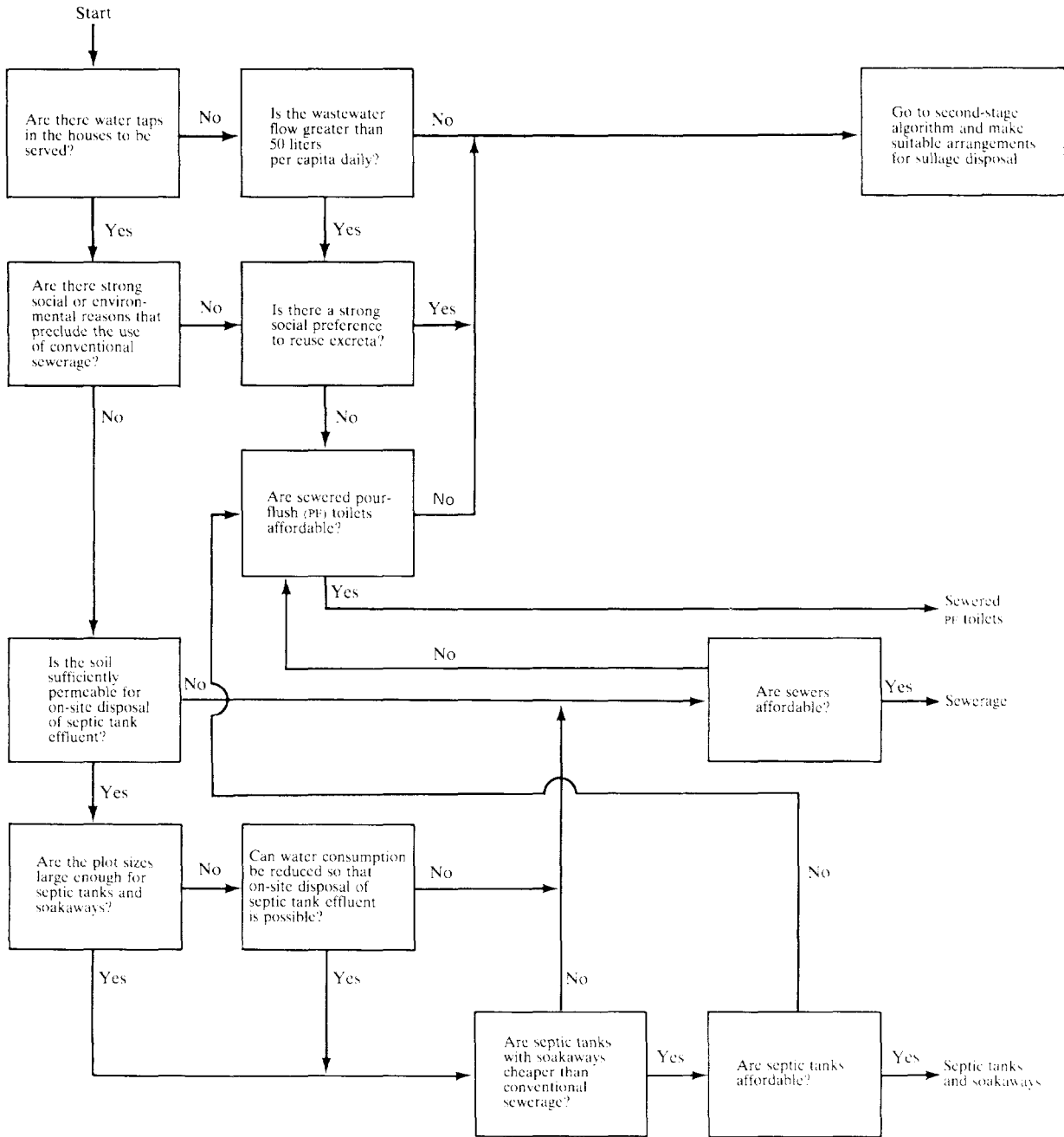
Figure 6-1. First-stage Algorithm for Selection of Sanitation Technology
