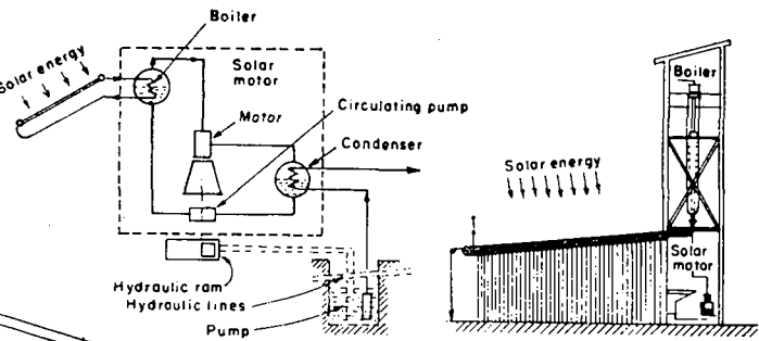
Figure 6. Solar pump (SOFRETES type)
