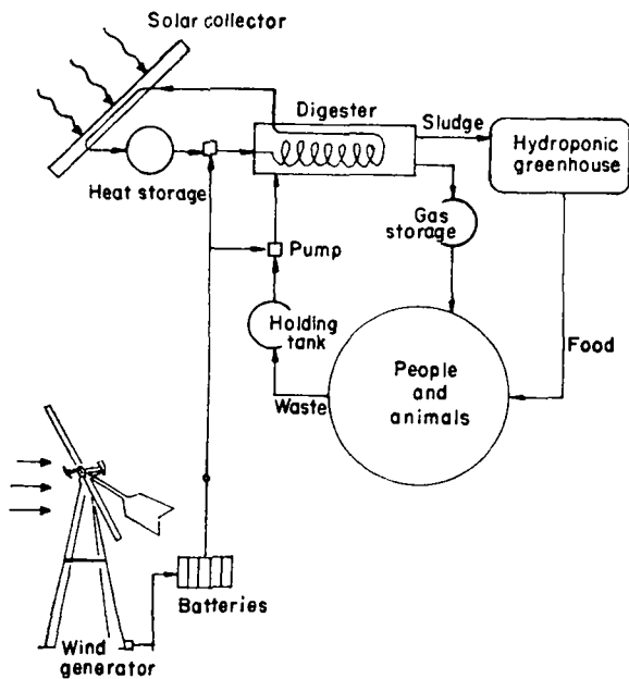
Figure 5. Maximum potential building systems
