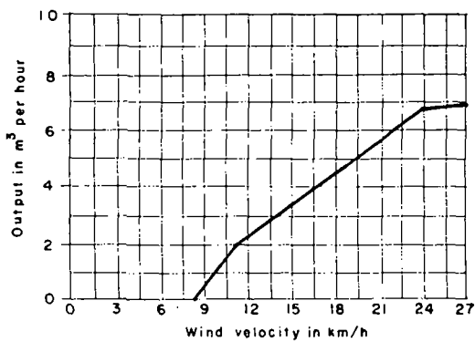
Figure 5. Wind pump performance
