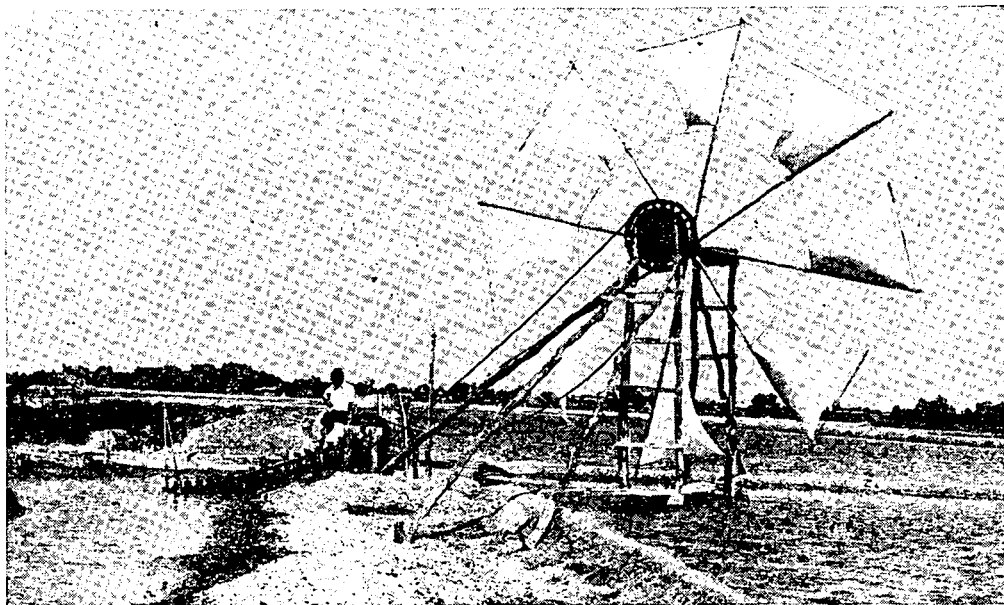
Figure 4. Cloth sail windmill
