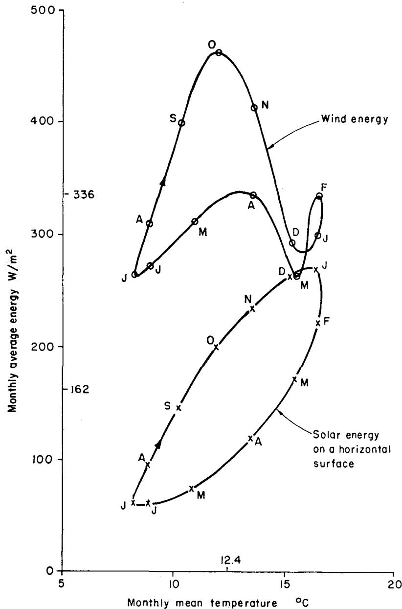
Figure 1. Wellington monthly average solar and wind energy
