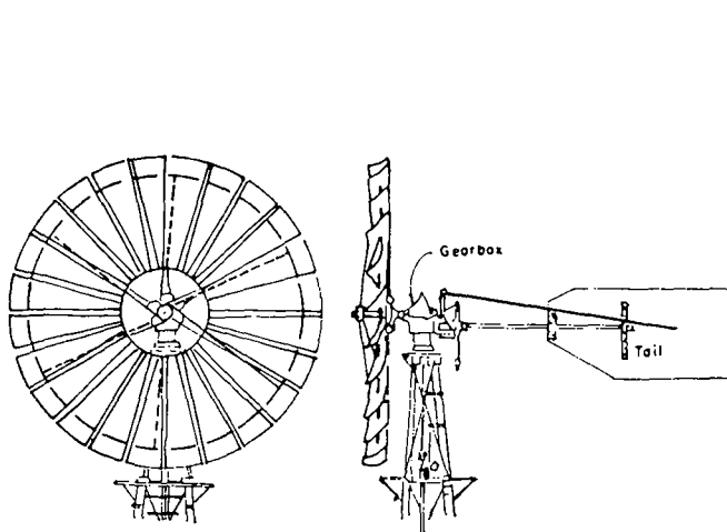
Figure 11. Multi-vane metal rotor
