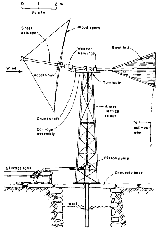
Figure 6. Greek sail rotor water pump
