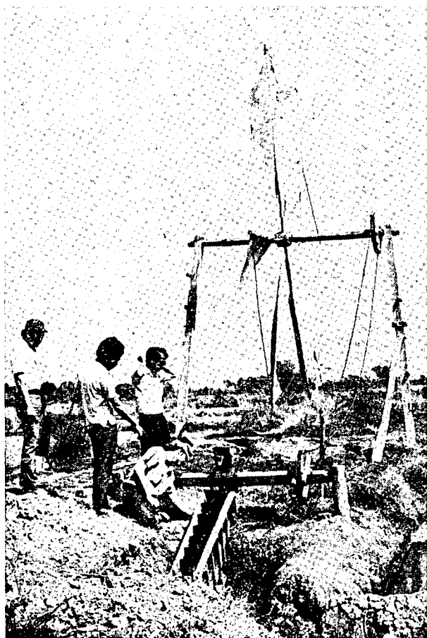
Figure 2. Bamboo-mat sail windmill
