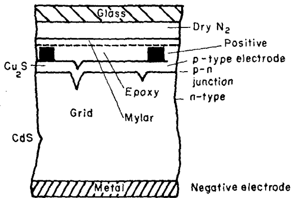
Figure 9. Cross-section of typical CdS/Cu 2 S solar cell
