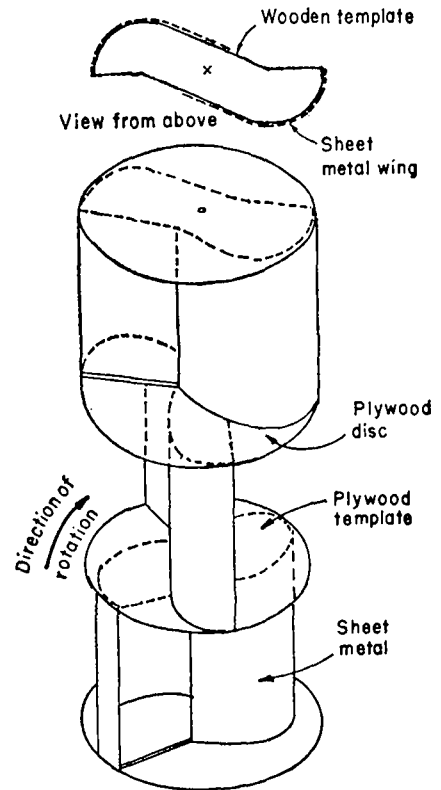
Figure 19. Three-tiered Savonius rotor
