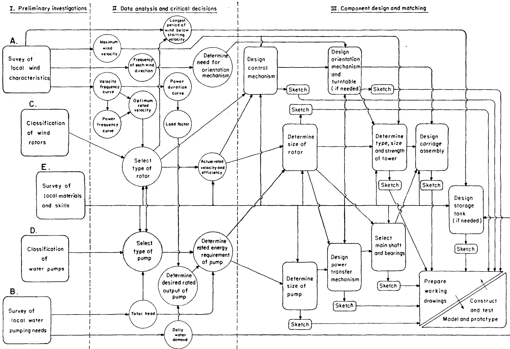
Figure 1. Sequential flow chart for design of water pumping windmill systems
