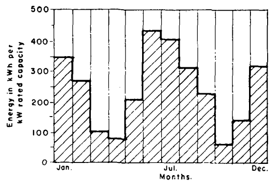
Figure 8. Monthly distribution of energy in the wind
