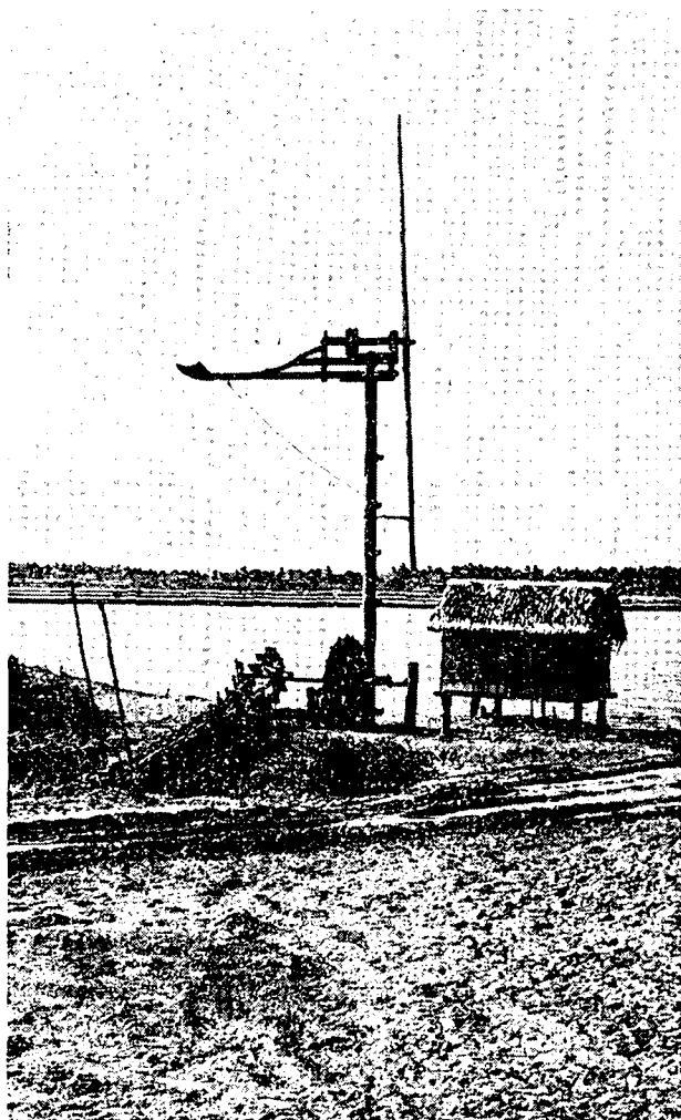
Figure 5. High-speed wooden-rotor windmill
