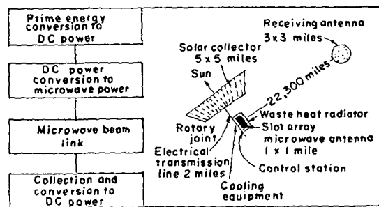
Figure 10. Satellite solar power system
