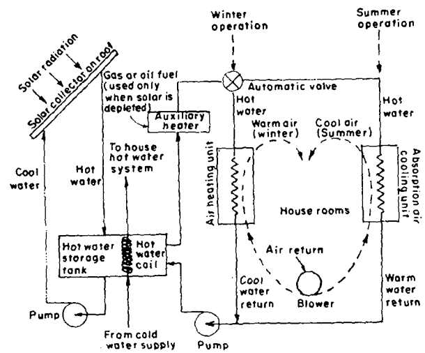
Figure 8. Residential heating and cooling
