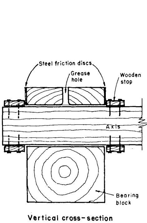
Figure 41. Double leg support bearing block
