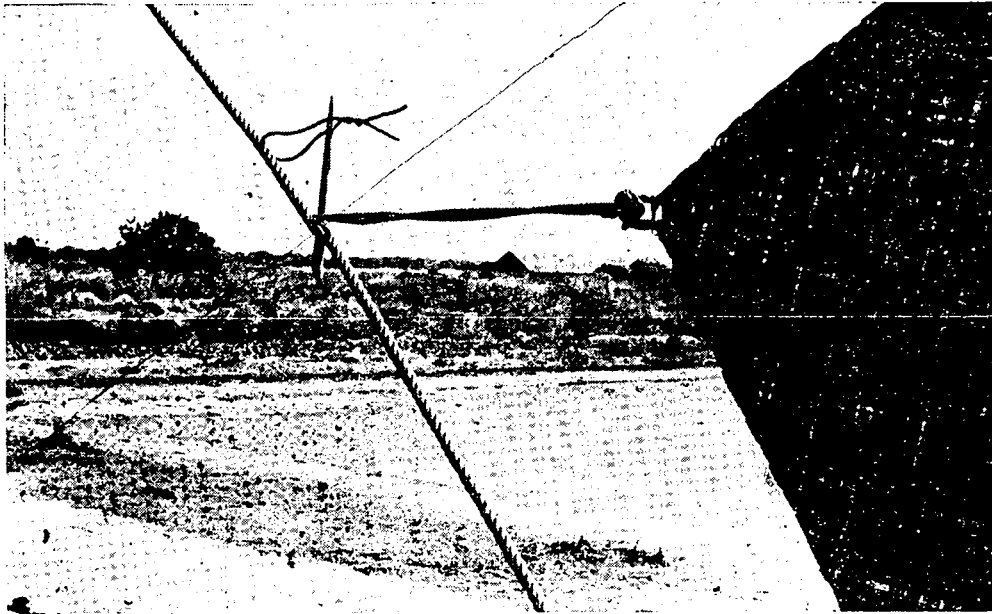
Figure 3. Quick-release sail-feeding device
