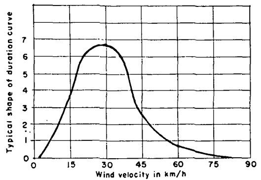
Figure 4. Velocity distribution (annual or monthly)
