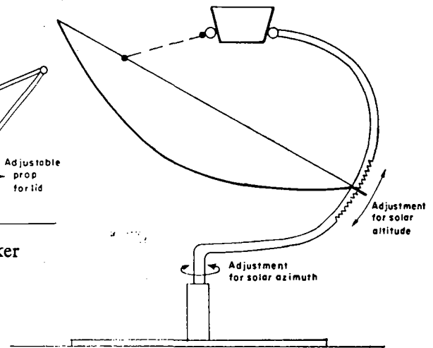
Figure 4. Solar cooker with parabolic mirror
