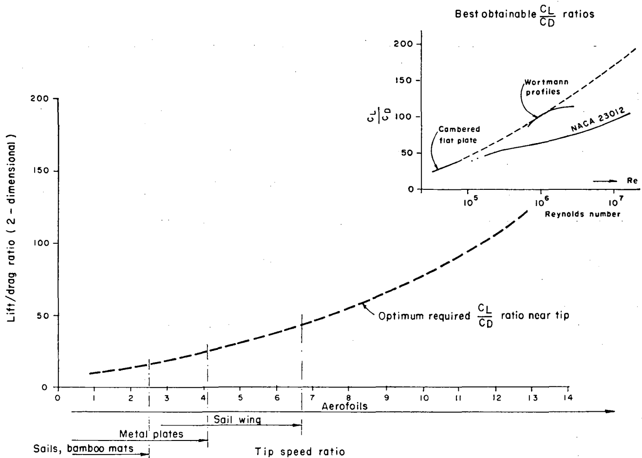
Figure 6. Lift/drag ratio
