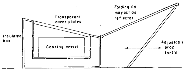
Figure 3. "Hot box" type of solar cooker
