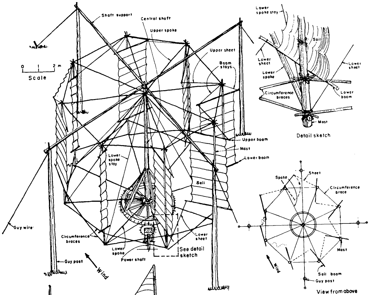
Figure 16. Chinese vertical-axis rotor
