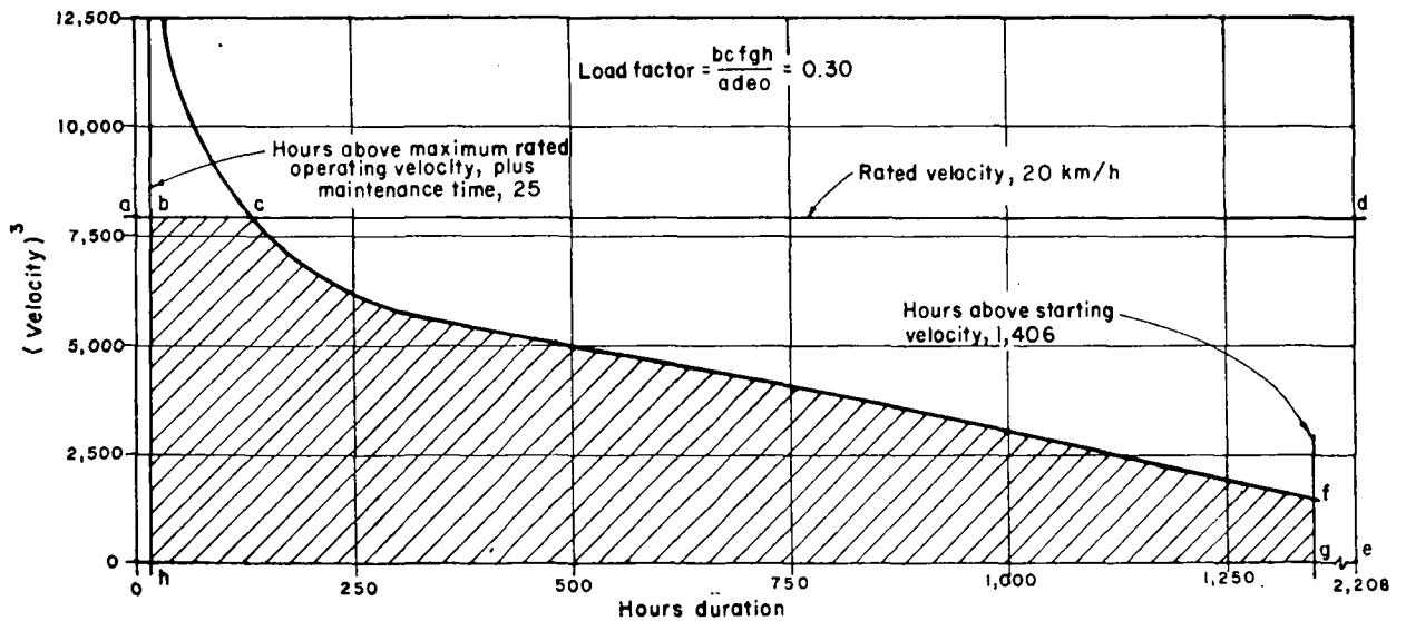
Figure 4. Shape of power duration curve
