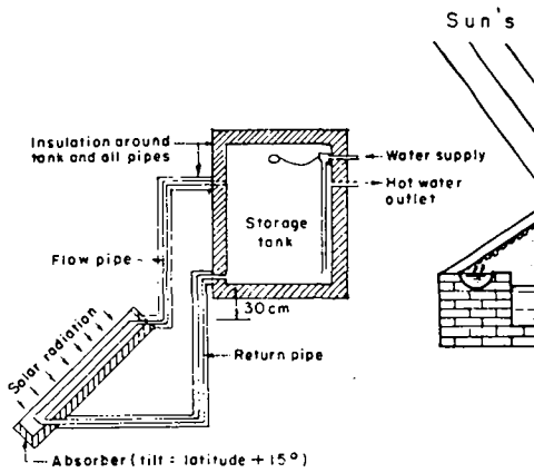
Figure 1. Domestic solar water heater
