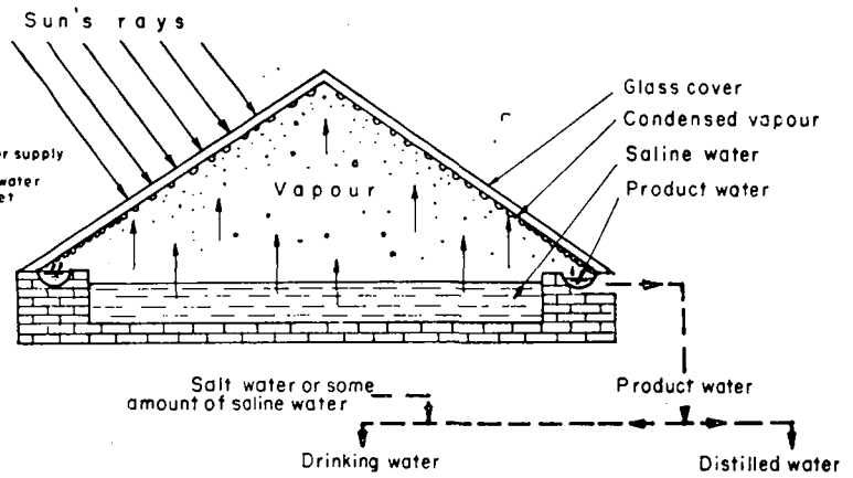
Figure 2. Solar still for water desalination
