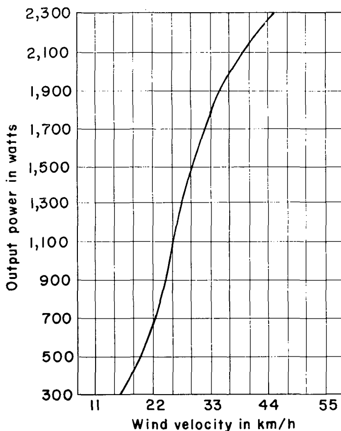
Figure 4. Output against wind velocity
