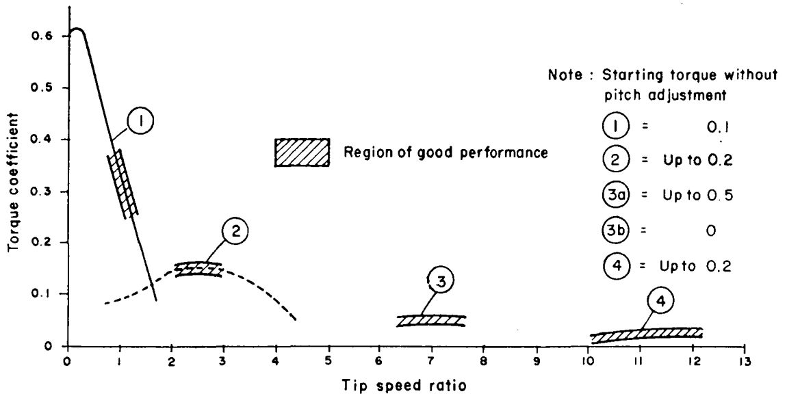
Figure 3. Torque coefficient
