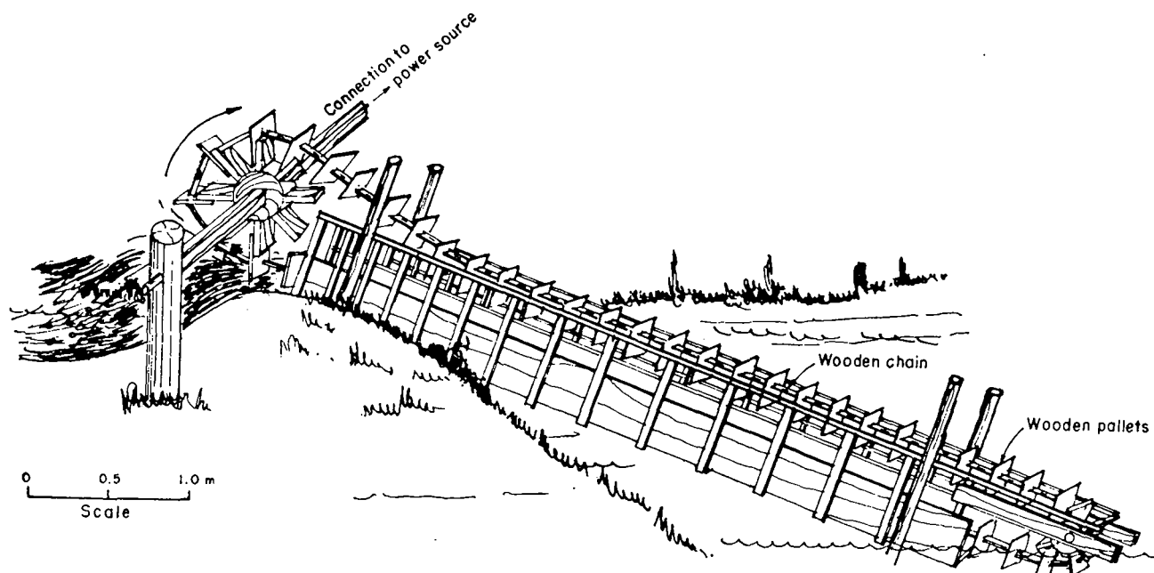
Figure 28. Wooden-pallet-type water pump
