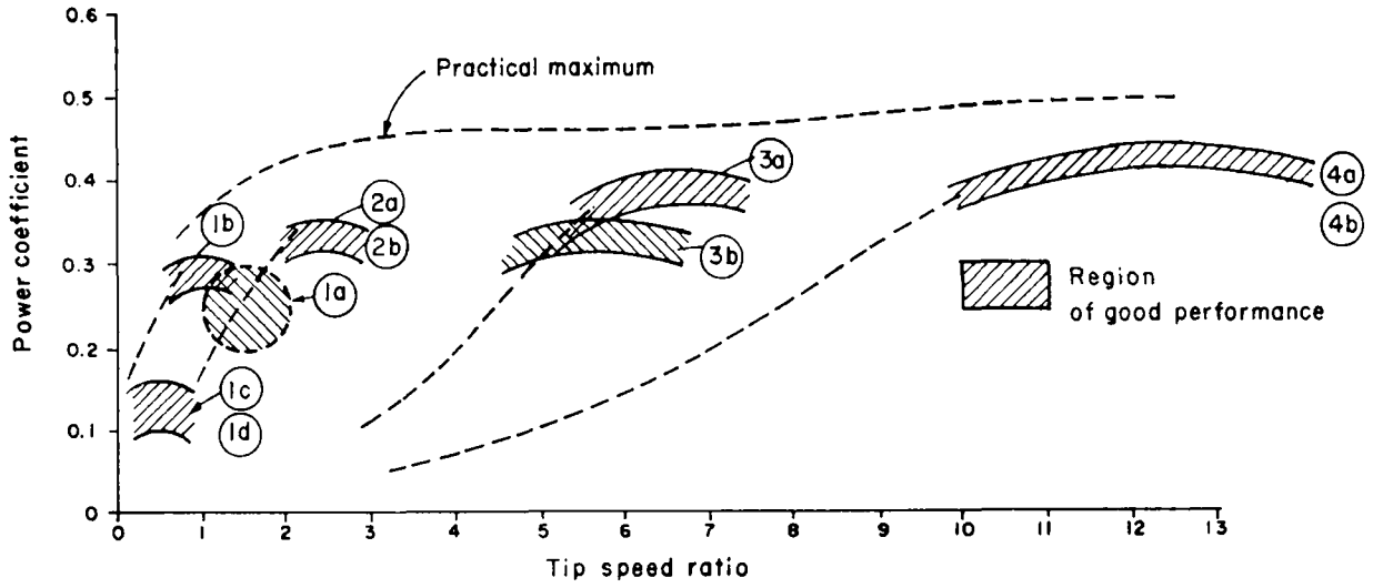
Figure 2. Power coefficient
