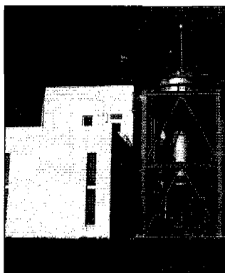
Commerically operational full-scale struvite recovery installation at Shimane Prefecture sewage works. Photo : Unitika Ltd, Japan.
