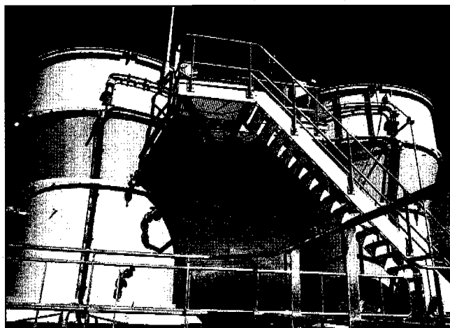
The full-scale calcium phosphate recovery installation at Geestmerambacht sewage works, The Netherlands, was visited by Conference participants. Photo : DHV, Amersfoort,
