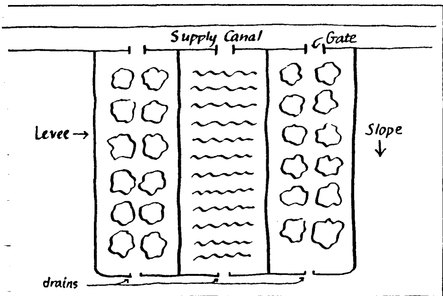
Border Irrigation
