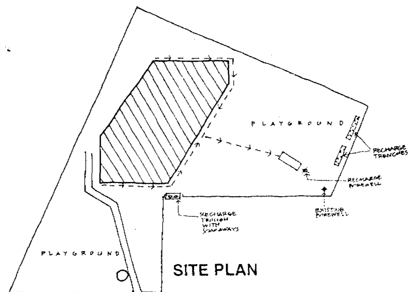
Figure 4.6.1 Scheme for water harvesting
