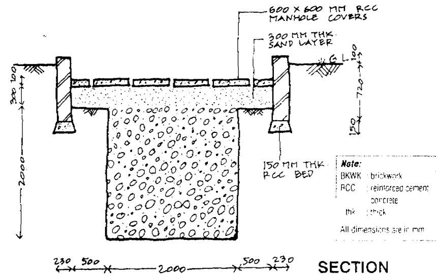
Figure 4.4.3 Details of recharge pit
