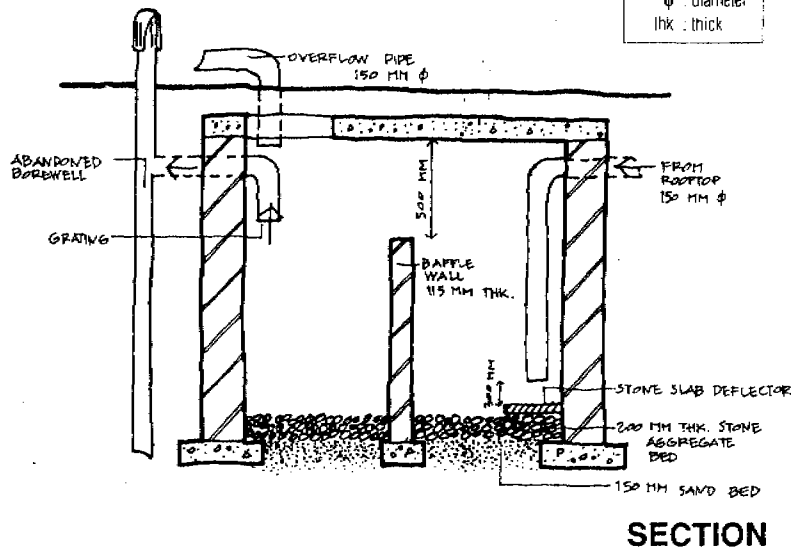
Figure 4.3.2 Details of recharge borewell and settlement tank
