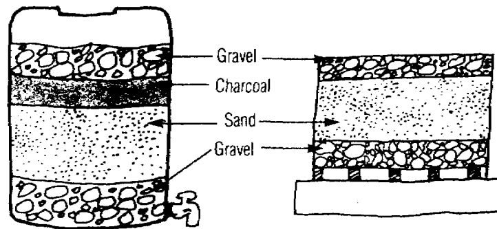
Composition of a charcoal filter
