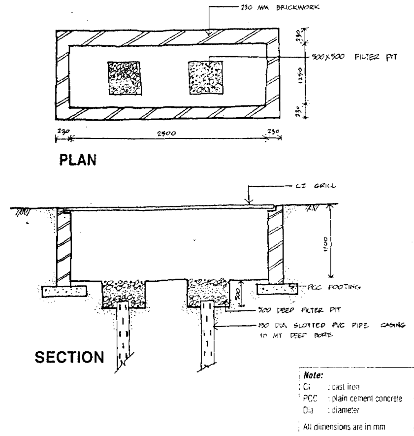
Figure 4.6.3 Details of recharge trough and soakaways
