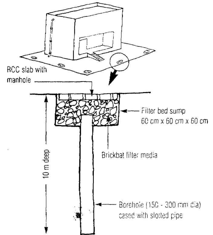
Figure 3.21 Location of soakaways in a building area with detailed section of soakaway
