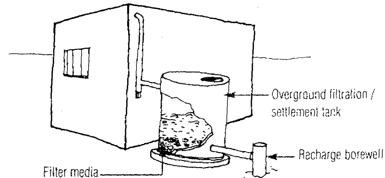
Figure 3.19 Overground PVC settlement tank
