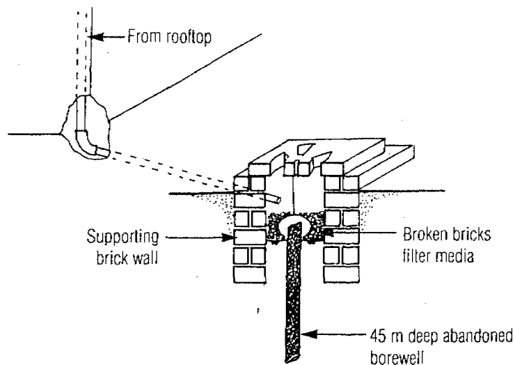
Figure 4.1.2 Detail of abandoned borewell recharging
