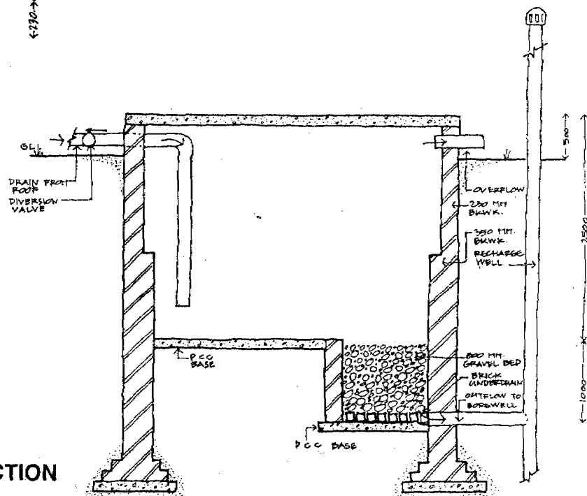
Figure 4.6.2 Details of recharge borewell and filtration tank
