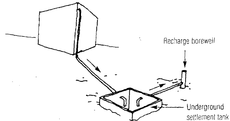
FIGURE 3.18 Underground masonry settlement tank
