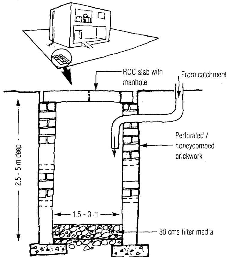
Figure 3.20 Location of recharge pit in a building area and detailed section of pit
