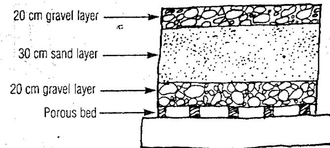
Figure 3.13 A simple sand filter which can be constructed at a domestic level
