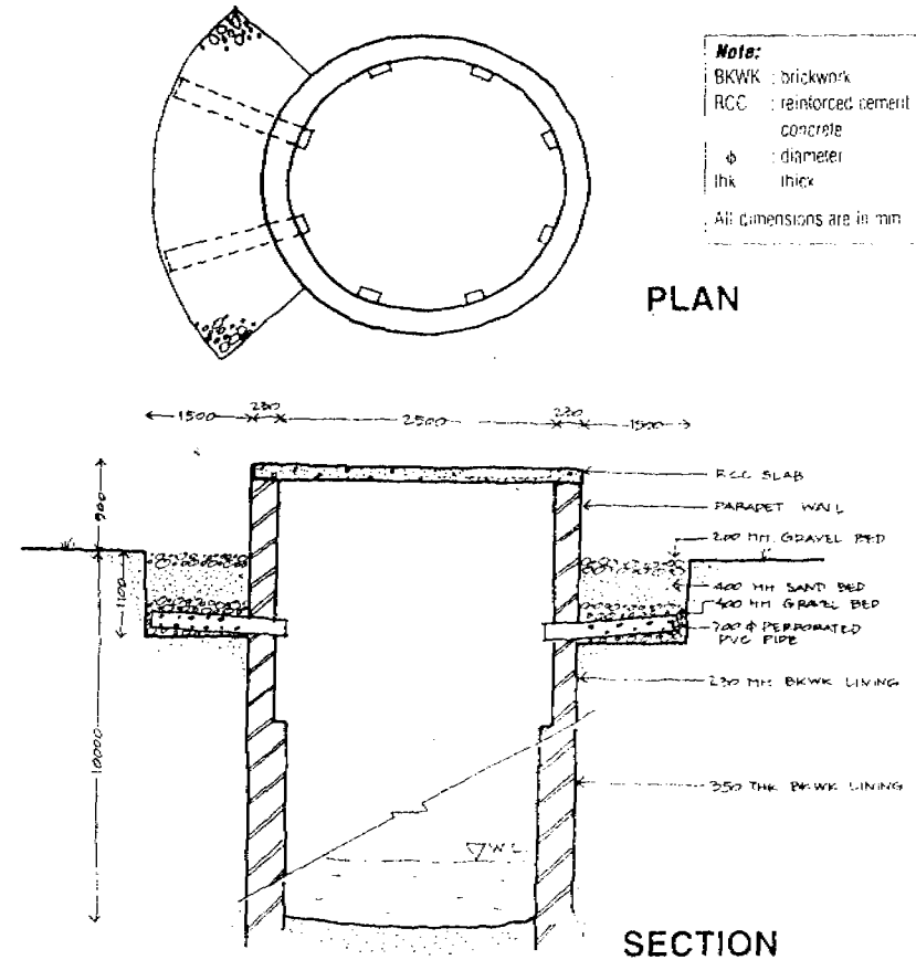
Figure 4.5.2 Details of recharge dugwell
