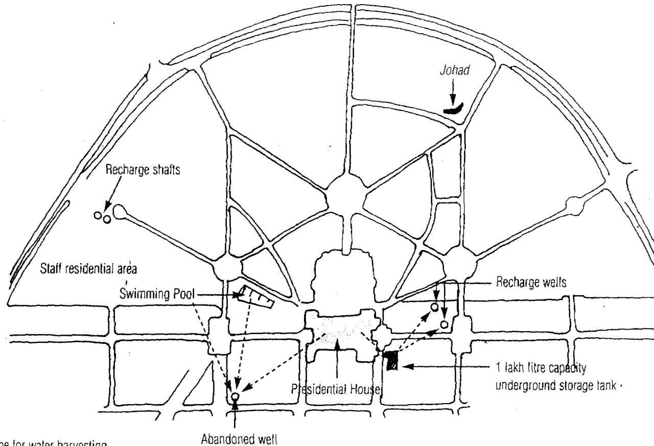
Figure 4.2.1 Scheme for water harvesting
