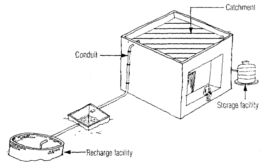
Figure 3.3 Elements of typical water harvesting system
