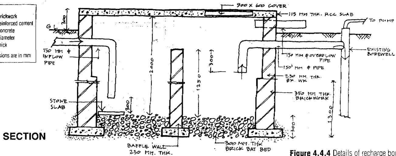
Figure 4.4.4 Details of recharge borewell and settlement tank
