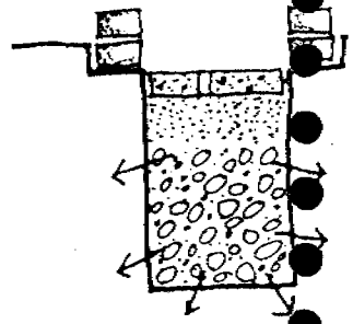
Figure 4.4.2 Details of recharge borewell
