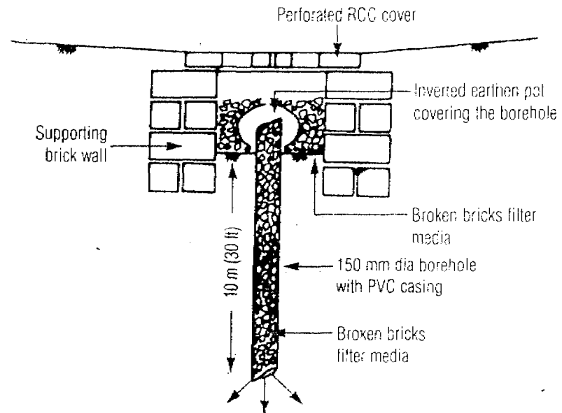
Figure 4.1.3 Detail of soakaway
