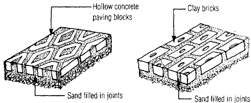
Figure 3.23 Permeable Pavements
