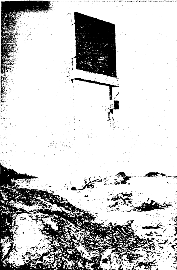
Figure 4. A standard 1 m 2 fog collector used for initial field investigations, Cerro Orara, Peru.
