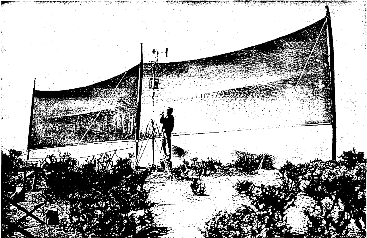
Figure 3. Two 4 m high by 12 m long fog collectors, and an upwind meteorological station, on the ridge at El Tofo, Chile.
