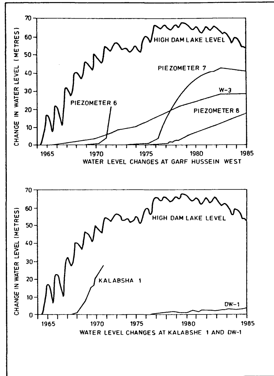
Figure 7.2 Groundwater head changes after the construction of the Aswan Dam
