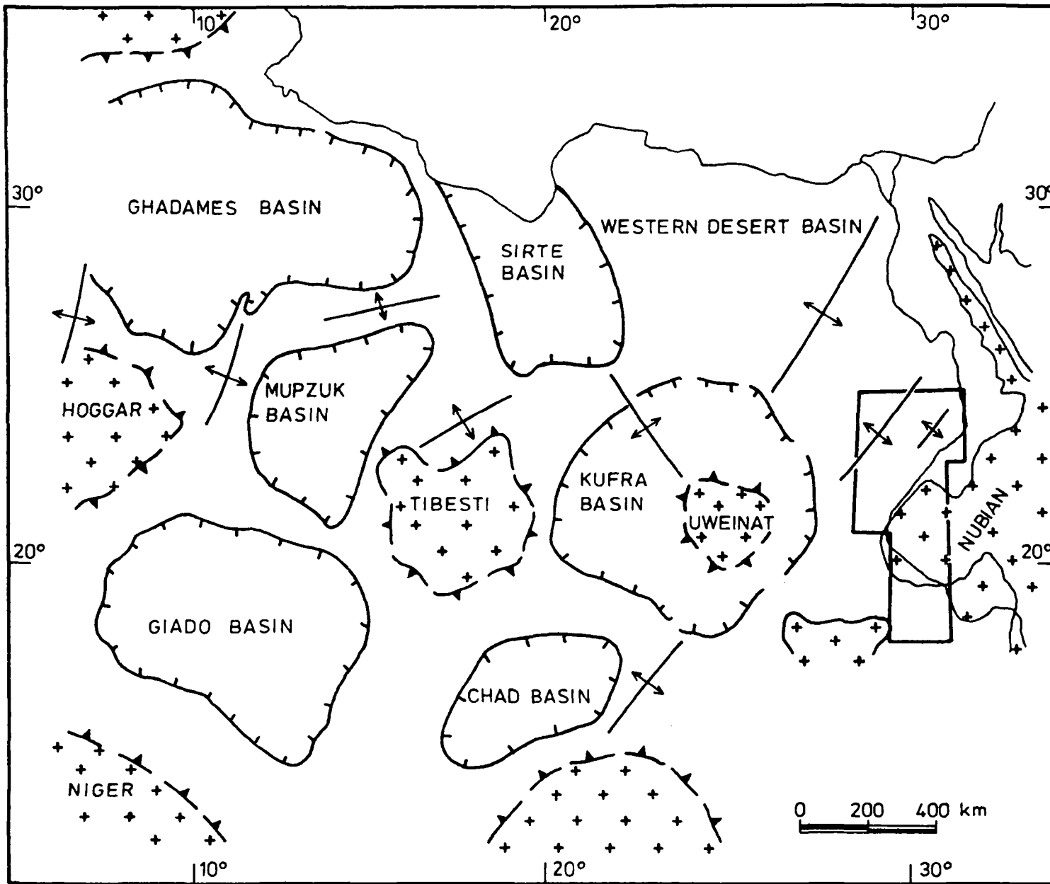
Figure 2.1 Regional geological basins in North-East Africa
