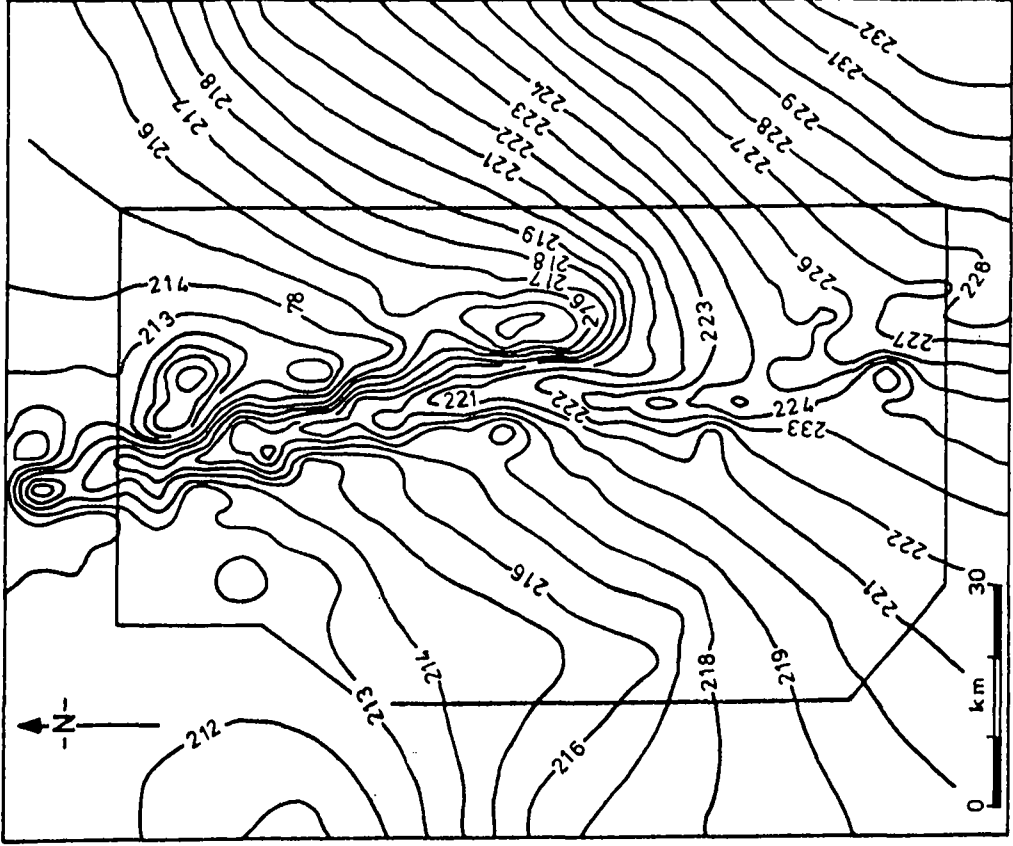
Figure 8.2 Groundwater head distribution adjacent to the Nile near Dongola simulated for abstraction of 760 \times 10^6 \text{ m}^3/\text{annum}
