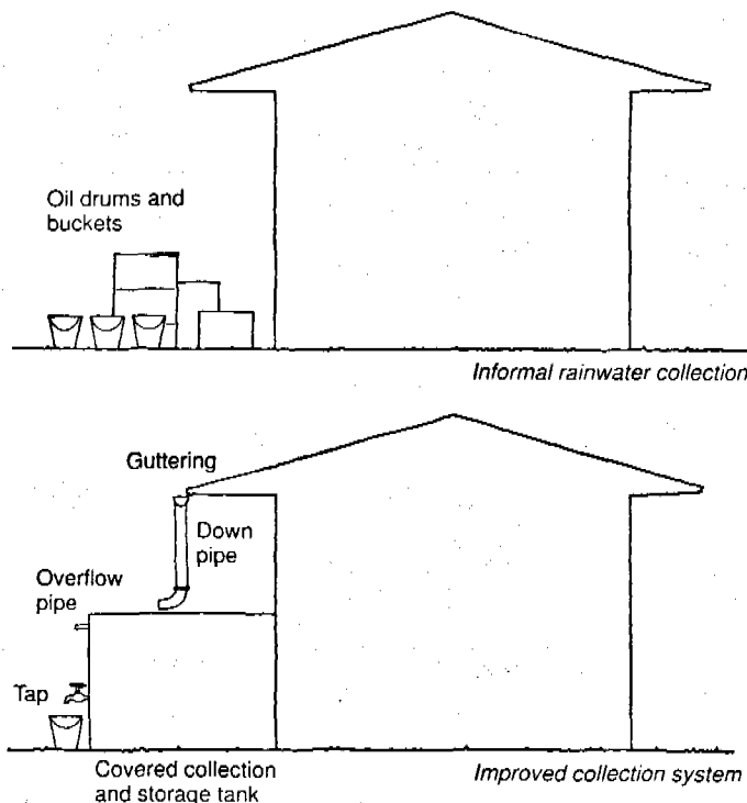
Fig. 2 Household rainwater collection.
