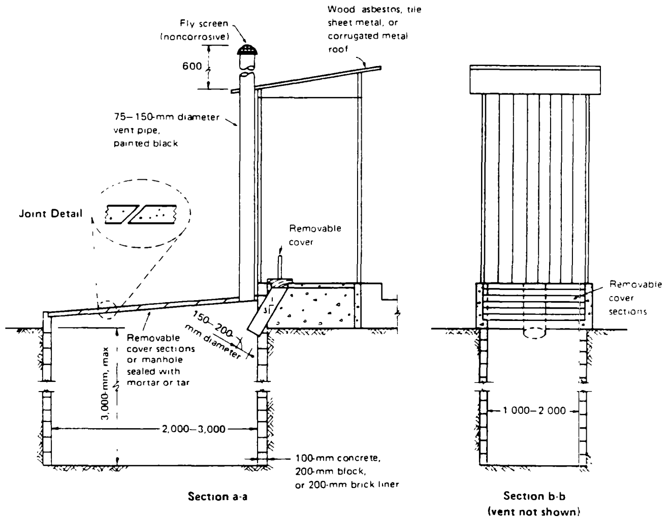
Illus. 21. Reed odorless earth closet (ROEC). (Source: Kalbermatten, et al., Appropriate Technology for Water Supply and Sanitation, Sanitation Field Manual. )
