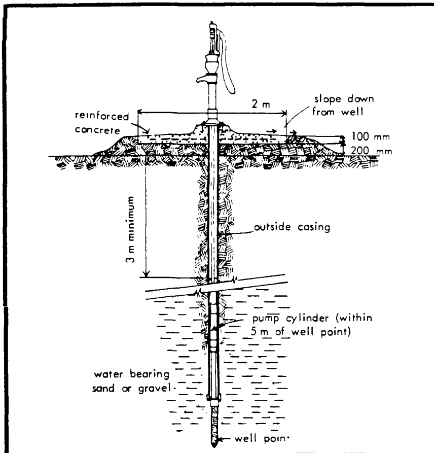
Illus. 16. A tube well with a driven well point. (Source: Cairncross and Feachem, Small Water Supplies .)
