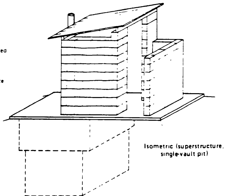
Illus. 20. Ventilated improved pit latrine (VIP). (Source: Kalbermatten, et al., Appropriate Technology for Water Supply and Sanitation. )
