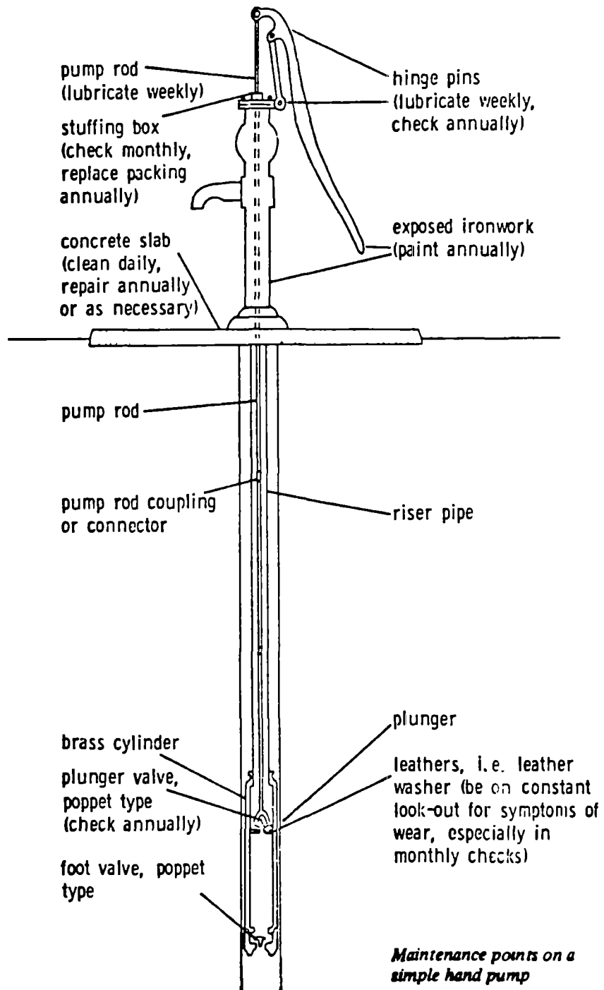
Illus. 25. Maintenance points on a simple handpump. (Source: Pacey, Handpump Maintenance .)
